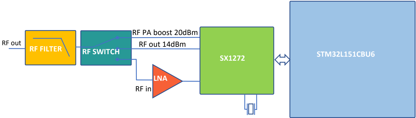
Figure 2: Module schematic
