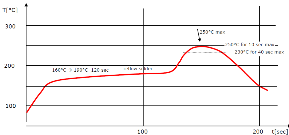
Figure 7: Reflow profile
